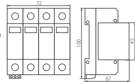
EL20C/4P / EL30B+C/4P
