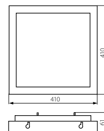
TYBIA LED 38W-NW
